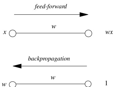
Fig. 7.14. Forward computation and backpropagation at an edge
