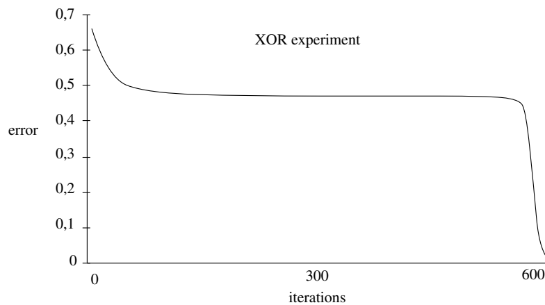
Fig. 7.23. Error function for 600 iterations of backpropagation
